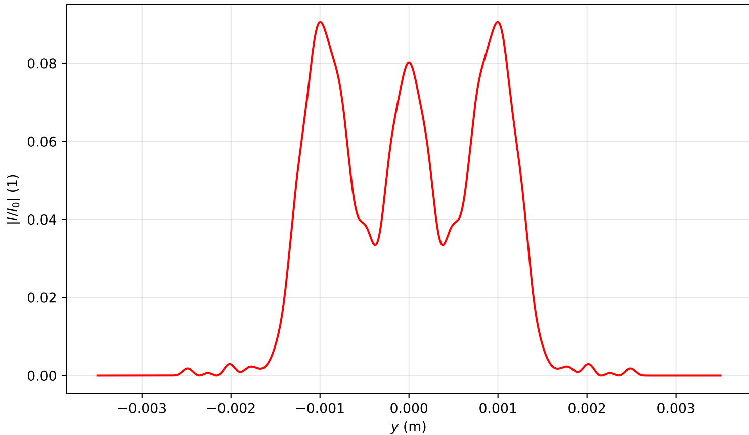
Intensity profile I(x=0, y, z=2.627)/I_0 , P_{in}=6.5P_{cr} , artificial time
